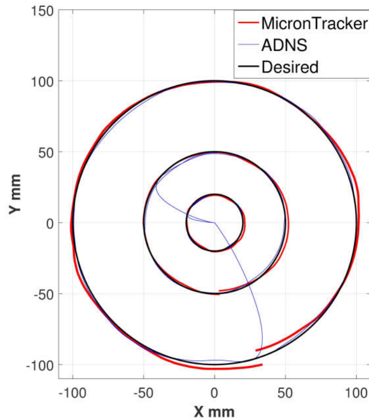
Figure 4.2: Circular Trajectories commanded and followed by the robot and measurement by ADNS sensors and Micron Tracker stereo camera.
