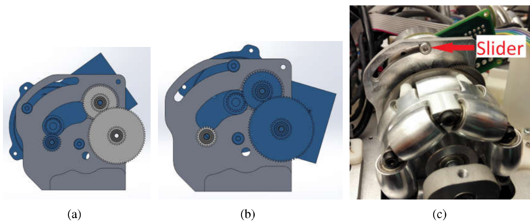
Figure 2.9: Power transmission mechanism at (a) low PTR (5:1); (b) high PTR (25:1) and (c) Custom made omni-wheels, gearbox and MAXON EC45 50W motor for mobile base
